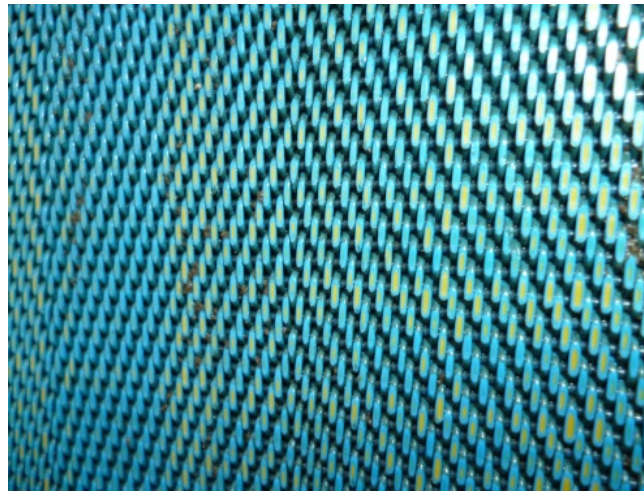
Picture 4: GKD offers the belt 1003 now with an integrated wear indicator to provide greater assistance in determining mechanical abrasion.
